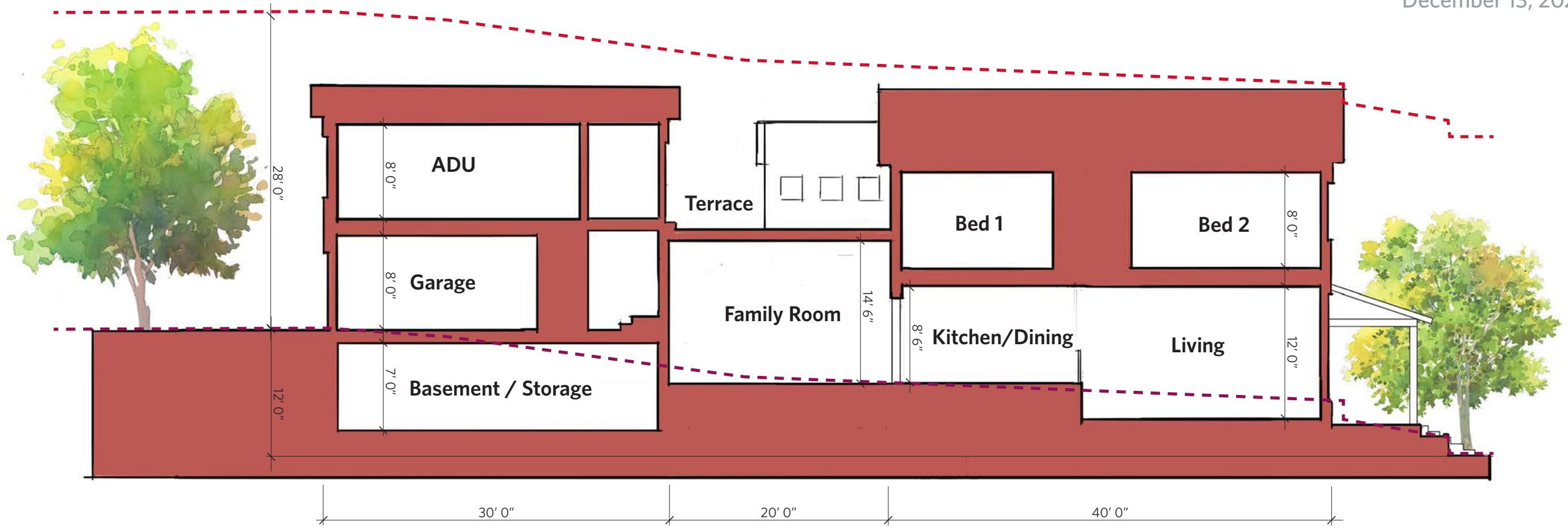
LOT SECTION
